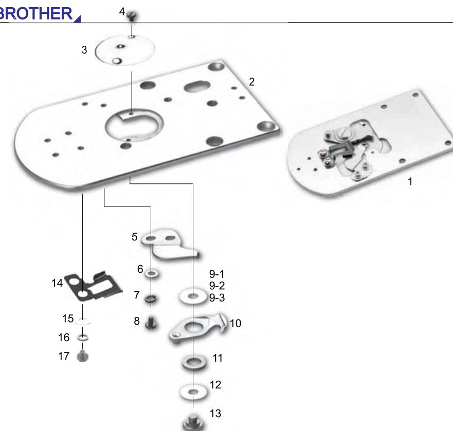
ASSEMBLY FOR BE-438F
