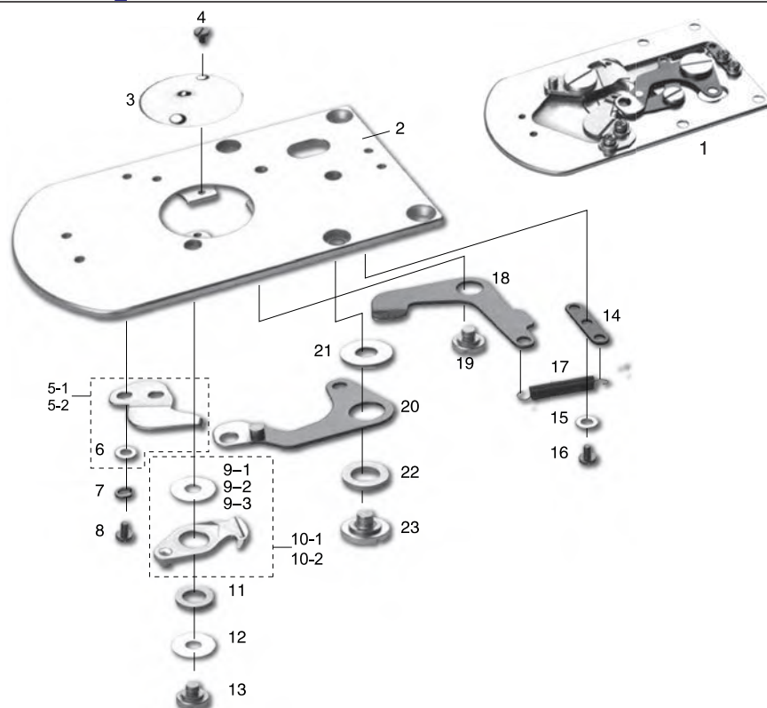
ASSEMBLY FOR BE-438D
