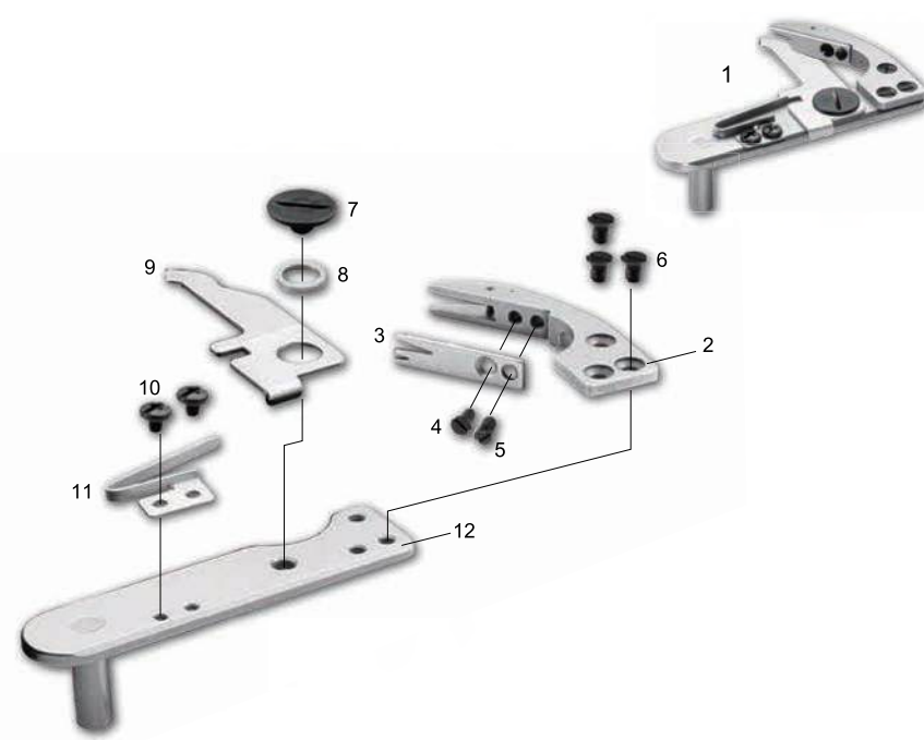
ASSEMBLY FOR RH-9820
