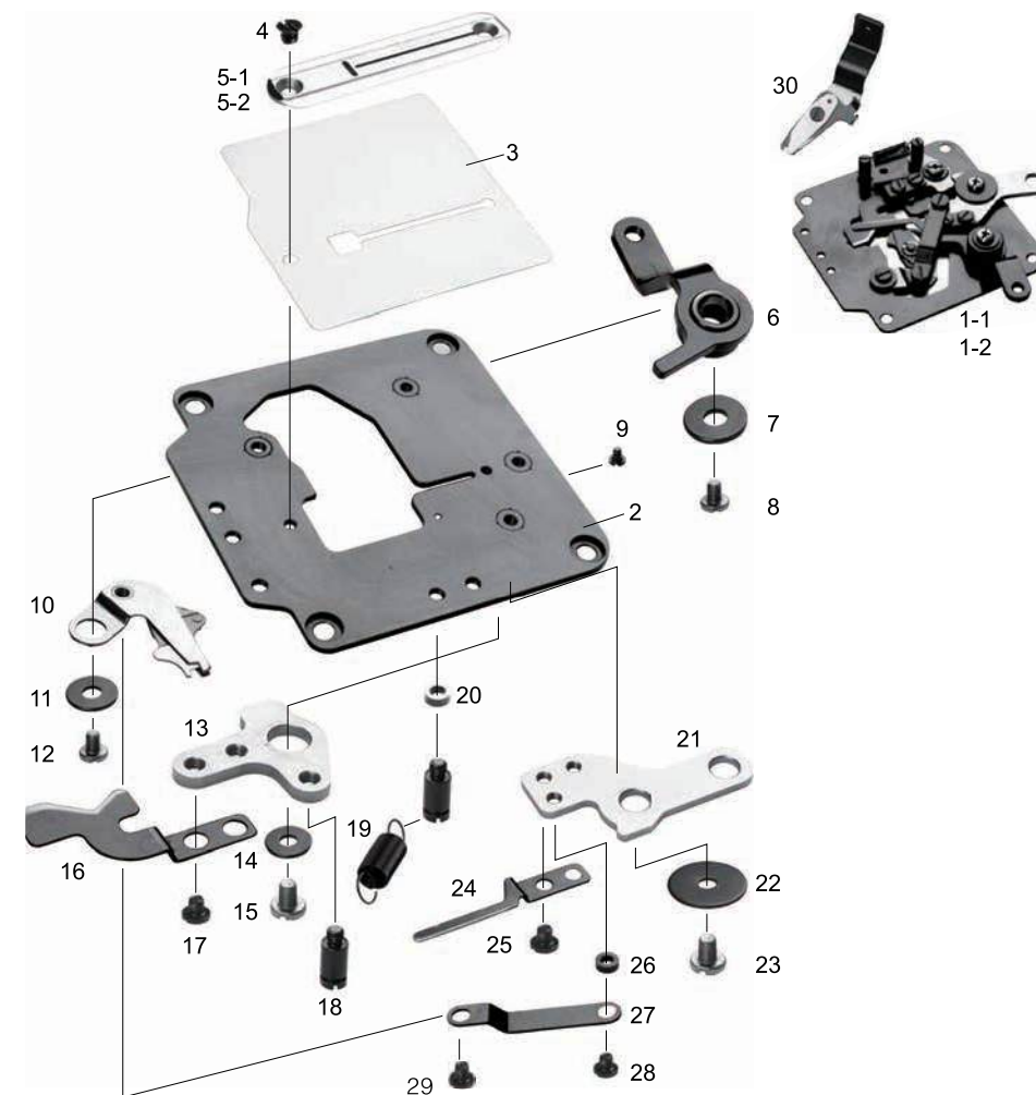
ASSEMBLY FOR LBH-1790
