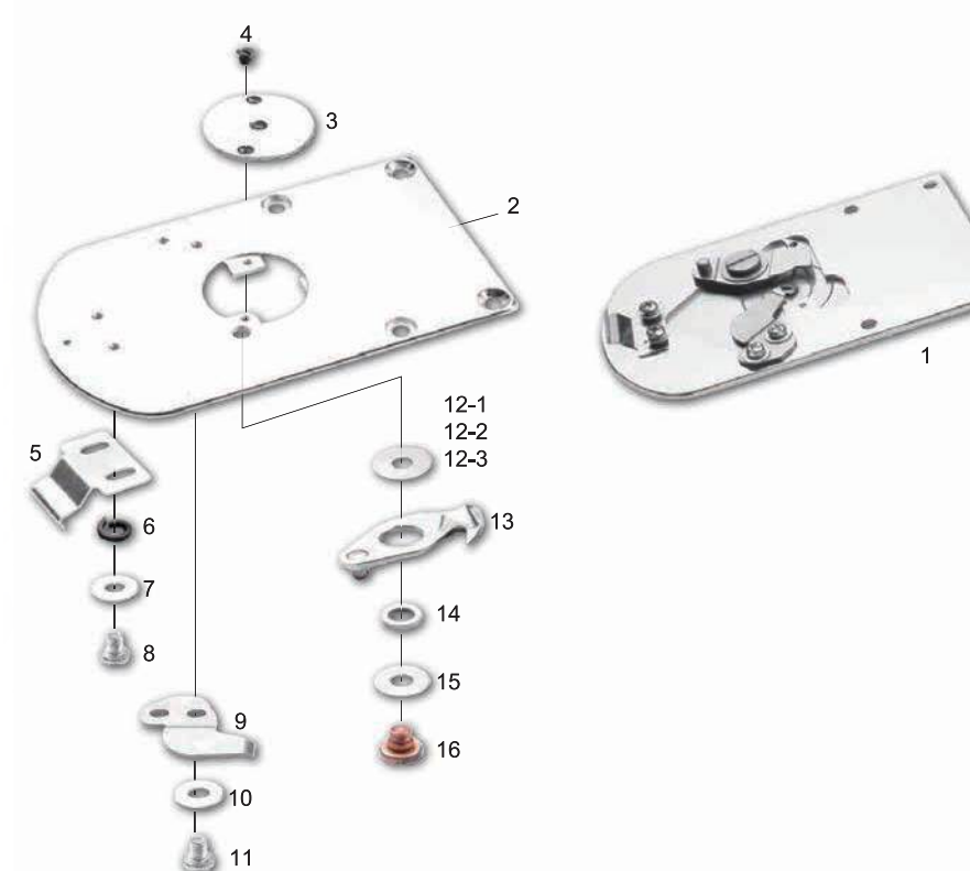
ASSEMBLY FOR BAS-311G
