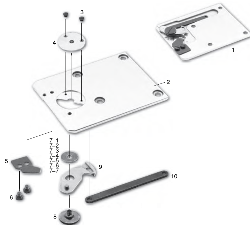
ASSEMBLY FOR MOL-254
