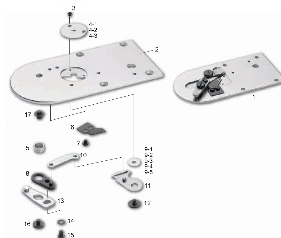
ASSEMBLY FOR LK-1850
